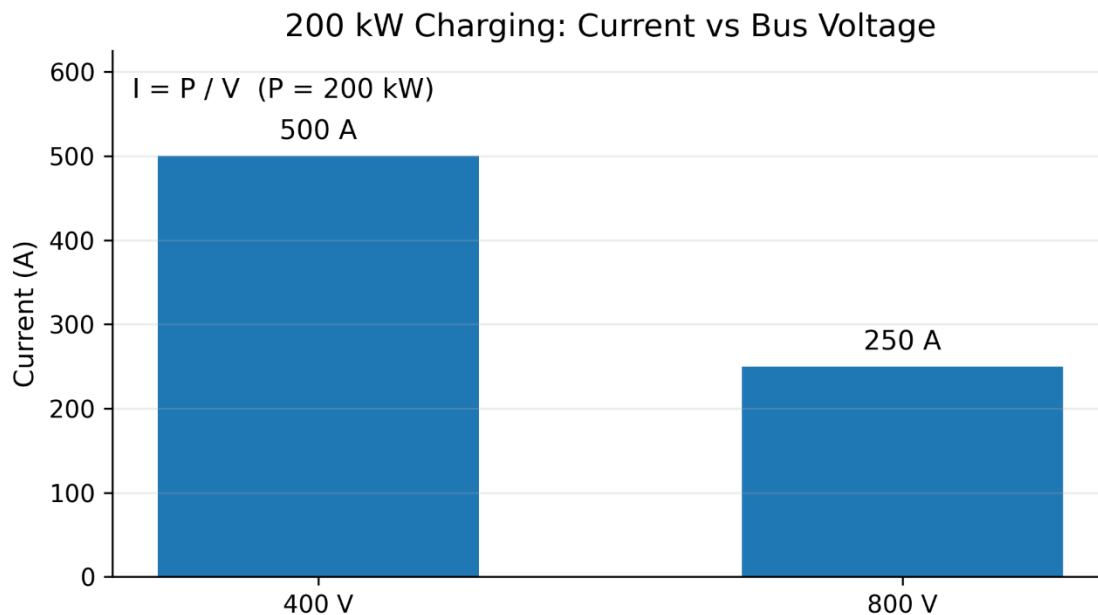
Fig. 4. Charging current and cable loss at 200 kW (400V vs. 800 V) [103]. (Exact values depend on cable specs, user can supply data for precise calculation.)
