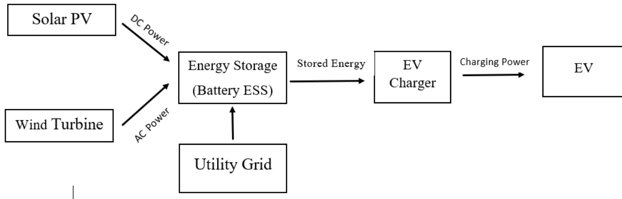
Fig. Renewable Energy Integration with EV Charging
