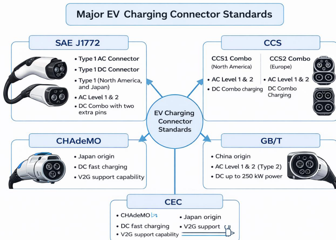
Fig. X. Major EV charging connector standards (based on [3],[6])
