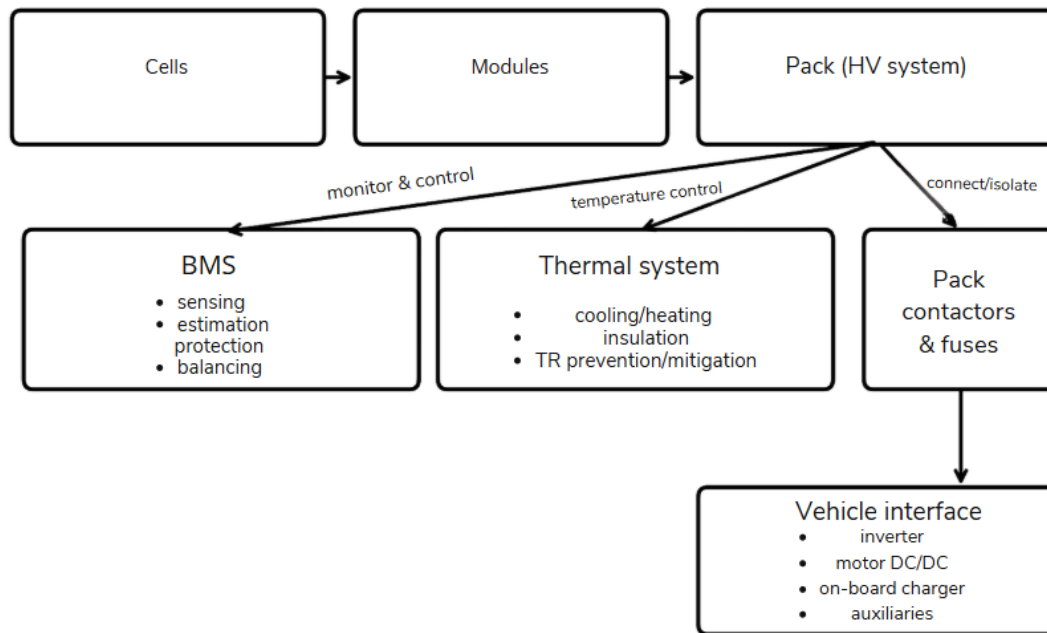
Fig. 2. Cell–module–pack hierarchy and key pack subsystems (BMS, thermal system, and contactors/fuses) that enable safe and reliable vehicle operation (created for this review).
